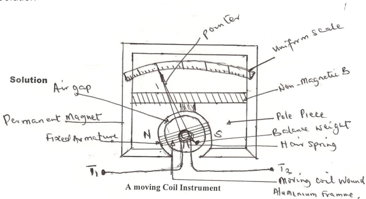
A moving Coil Instrument
